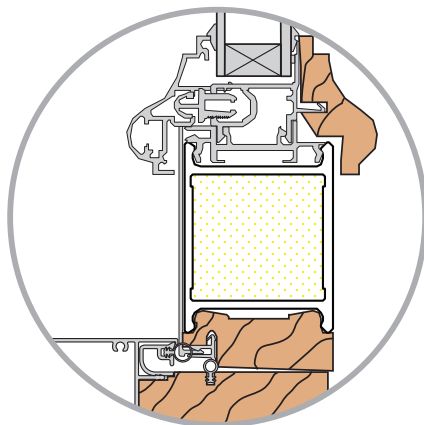
Narrow stile for garden and classic terrace door
