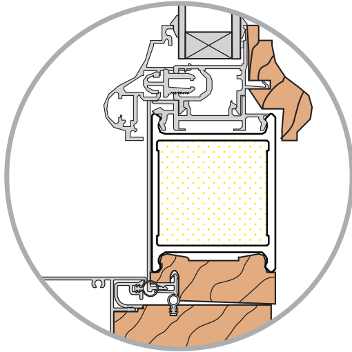
Narrow frame (glass garden door) Traditional type molding
