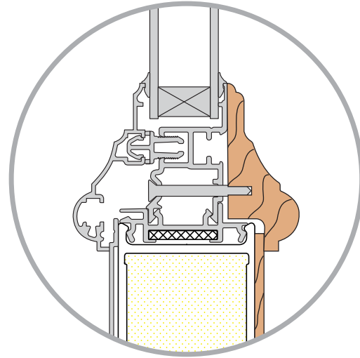
"AT" molding traditional glass
