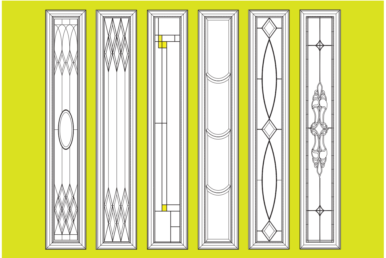
Sidelight standard dimensions (without base)
