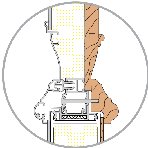
"A" molding traditional panel
