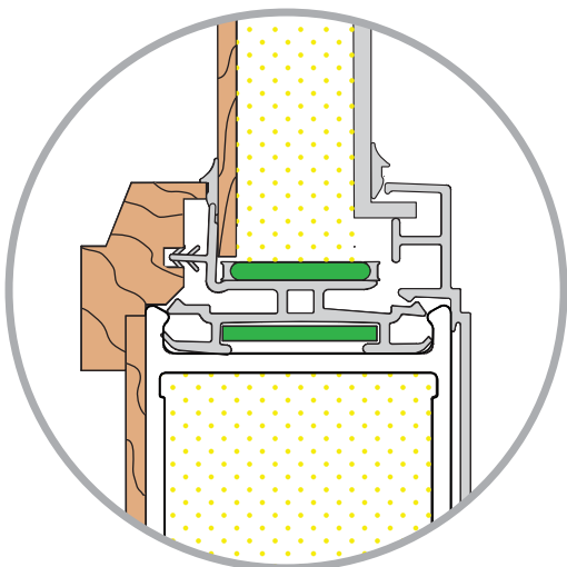
Modern type molding Glass or panel
