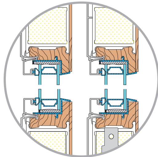
Lift and slide door
