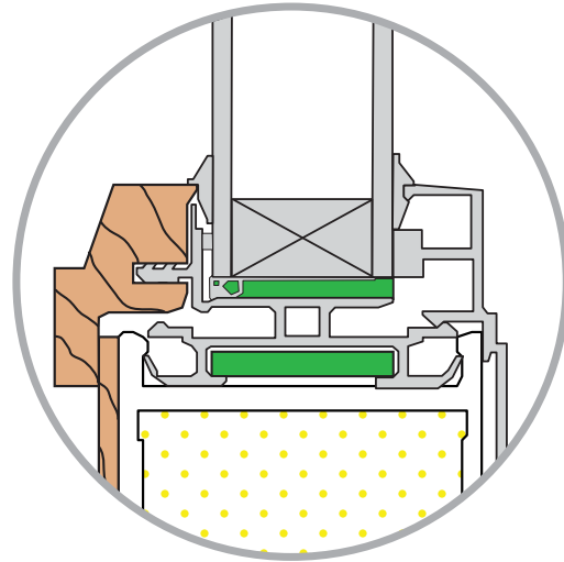
Narrow frame (glass garden door) Modern type molding
